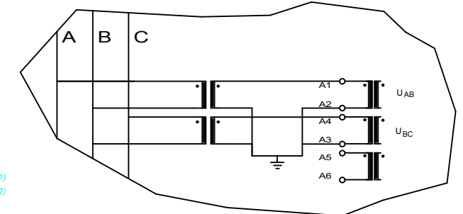
2TT'S CONNECTION CONEXION PARA 2TT'S
